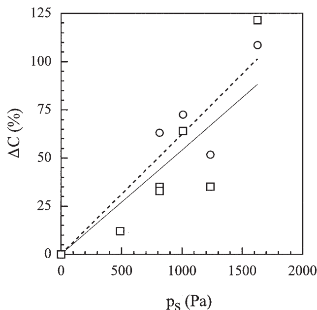
Figure 6. Percent change in effluent dissolved TCE concentration as a function of p_s (here x=0.15 m, \phi=245 Hz).
